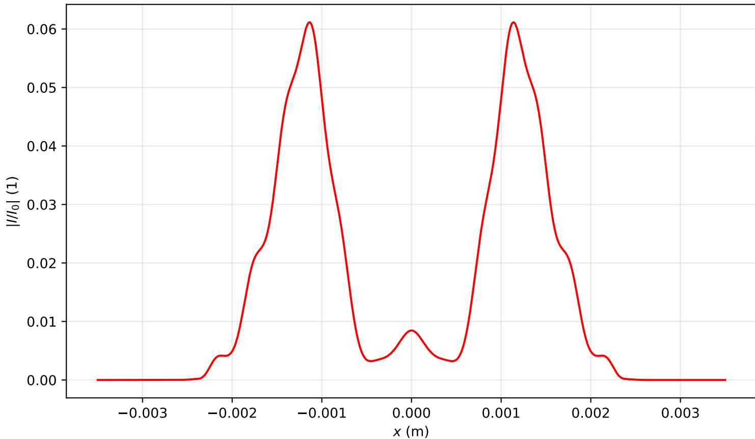
Intensity profile I(x, y = 0, z = 3.582)/I_0 , P_{in}=6.5P_{cr} , artificial time
